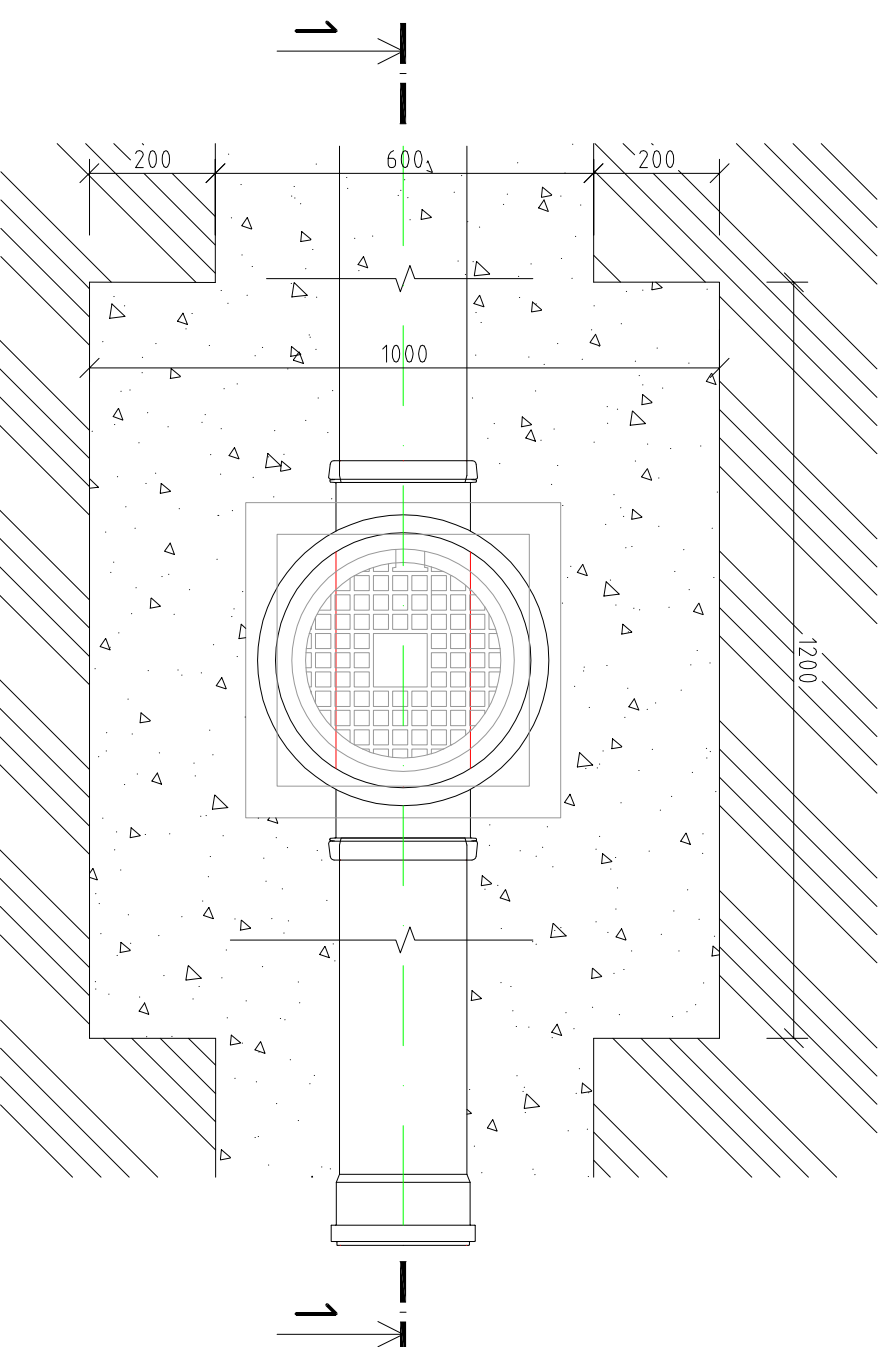
PVC šachta Š1, Š2 DN 400 d 200
