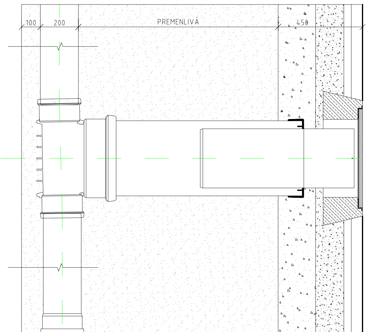
REZ 1-1
